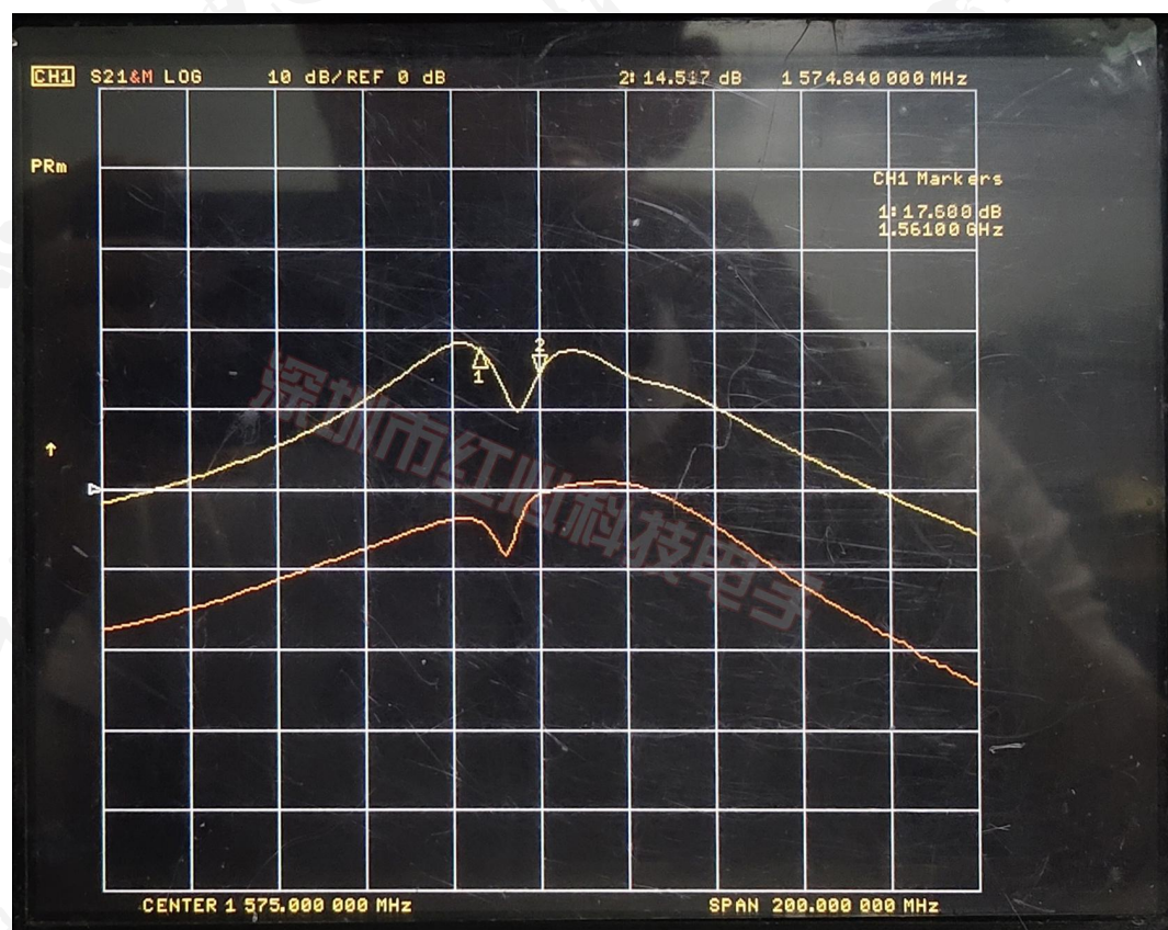
(Gain)增益图
