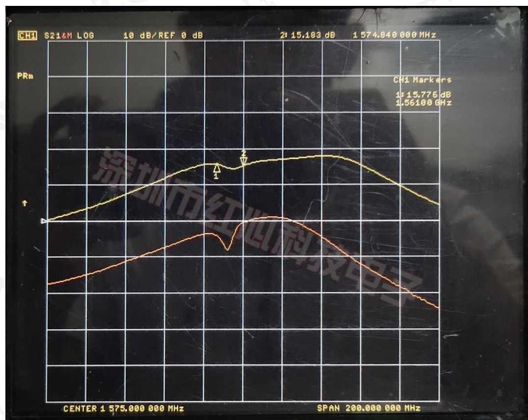
(Gain)增益图
