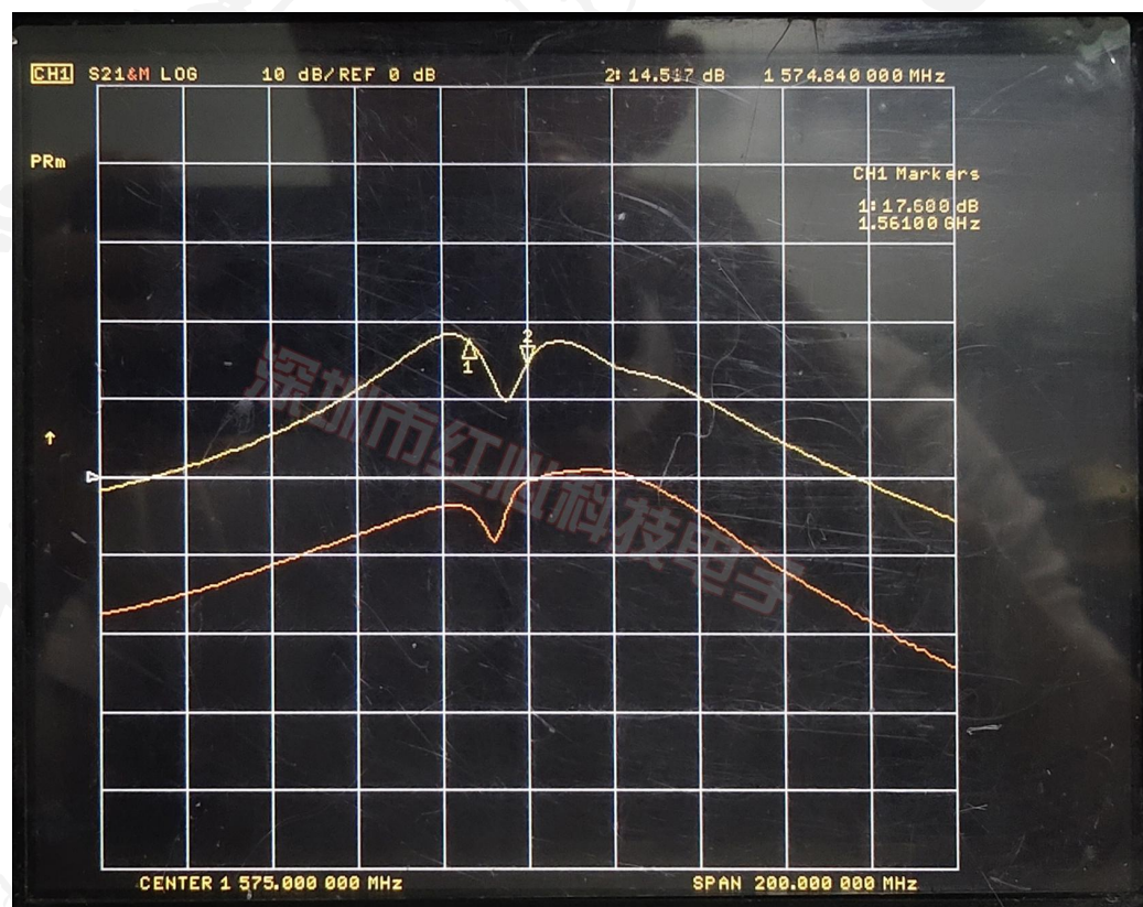
(Gain)增益图
