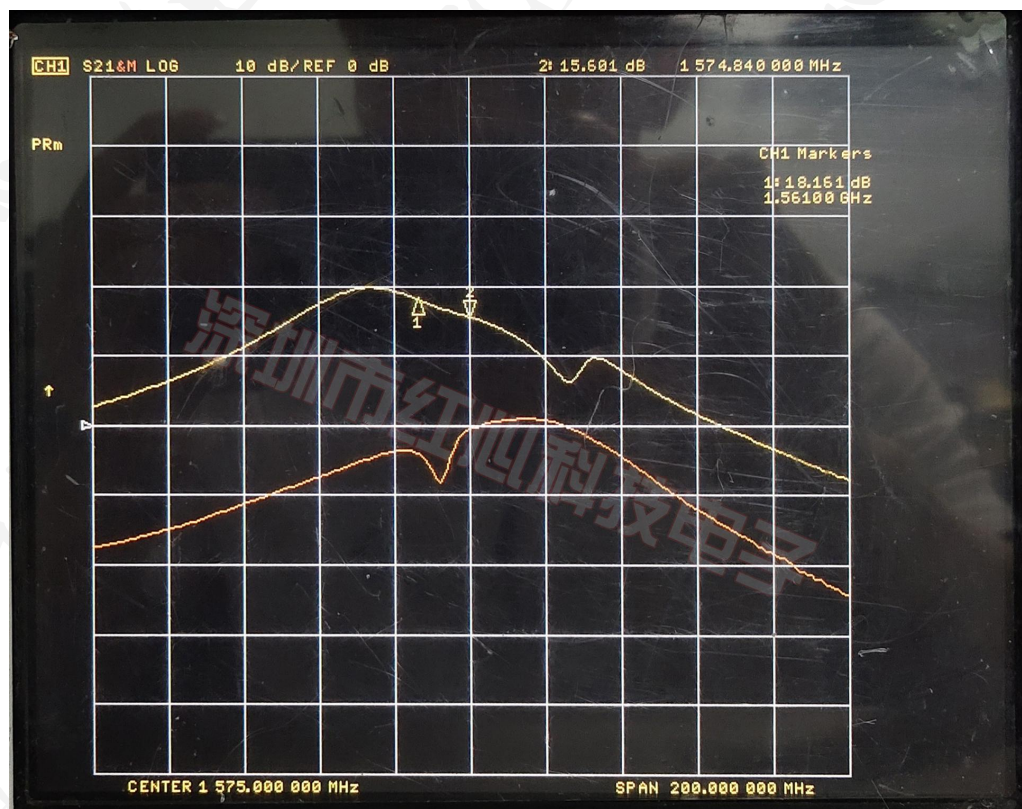
(Gain)增益图
