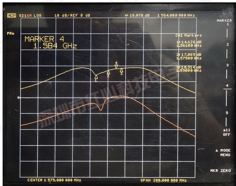
(Gain)增益图
