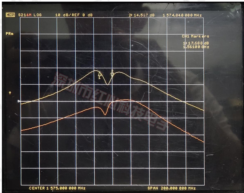
(Gain)增益图
