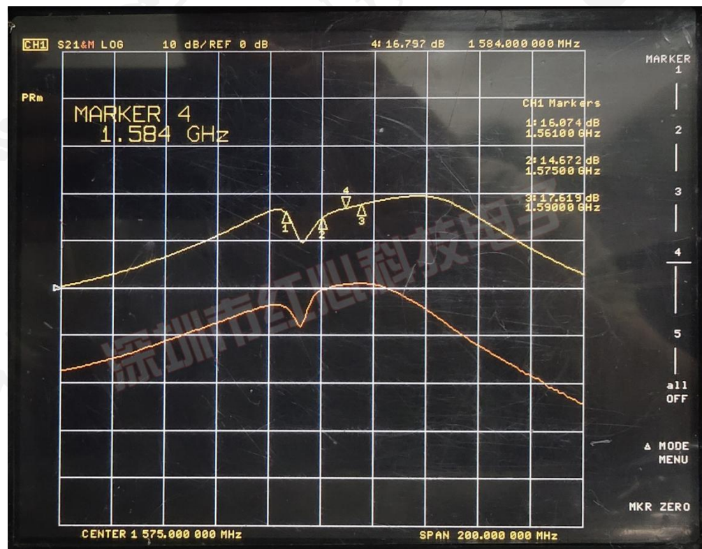
(Gain)增益图
